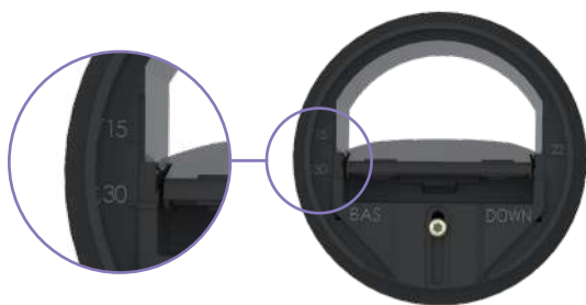
Example of an adjustment at 30 m 3 /h: regulator set at the '30' mark on the left
